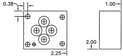
D03 SERIES CIRCUIT COVER PLATE PART NO. BY-CS
